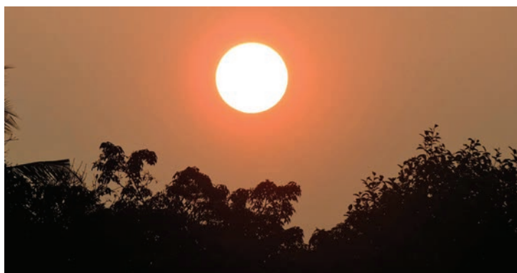
Fig. 12.6: The rising Sun
