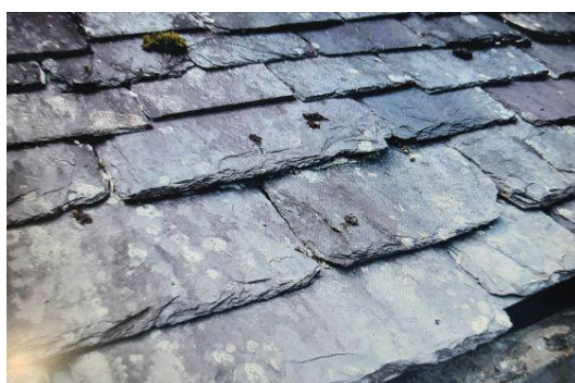
Fig. 11.6: Rocks used for roofing
