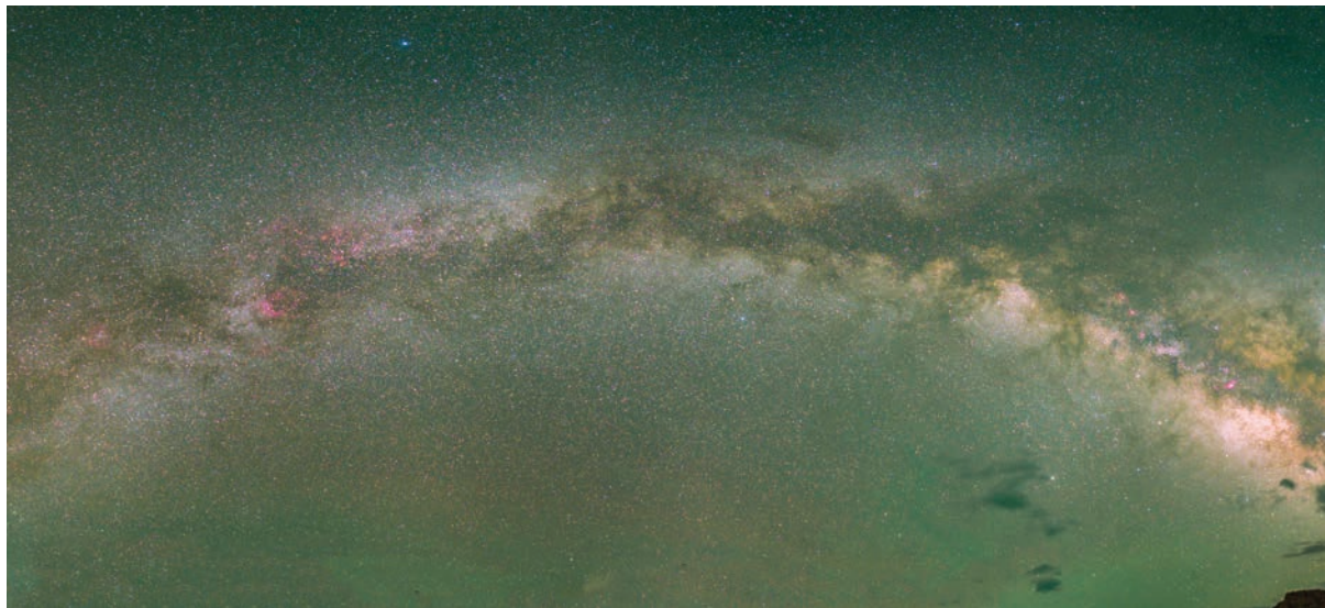
Fig. 12.11: Milky Way Galaxy as seen from a very dark location in Ladakh, India
