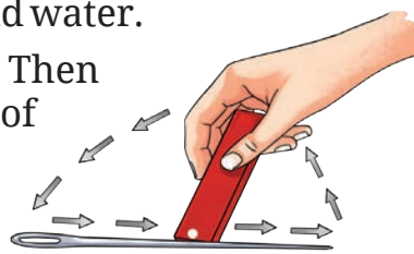
Fig. 4.7(a): Making an iron needle a magnet
