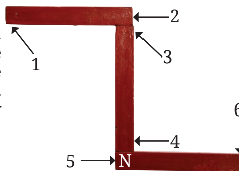
Fig. 4.17: Three bar magnets
