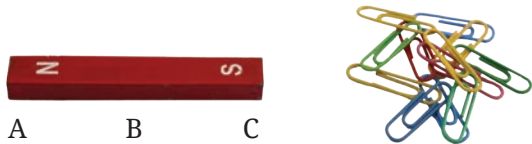
Fig. 4.15: Bar magnet and heap of steel U-clips
