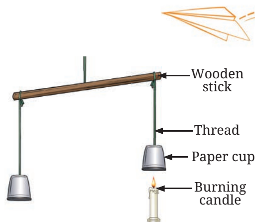
Fig. 7.3(b): Hot air rising up
