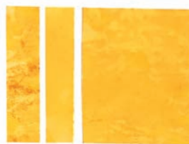
(b) Turmeric paper strips
