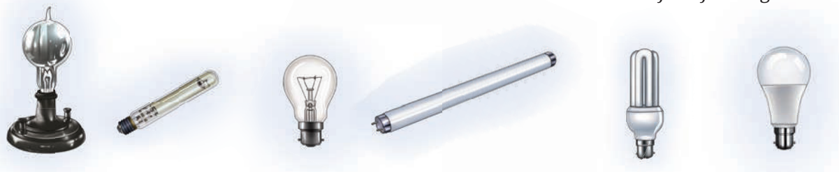
Fig. 11.3: Some sources of electric light
