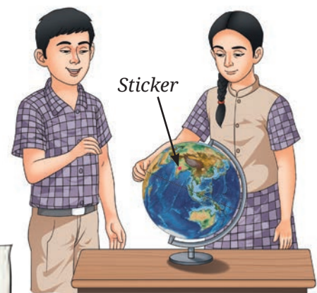
Fig. 12.4(a): Using a globe to understand rotation of the Earth
