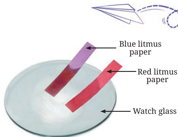
Fig. 4.7(d): Testing of solution with litmus papers
