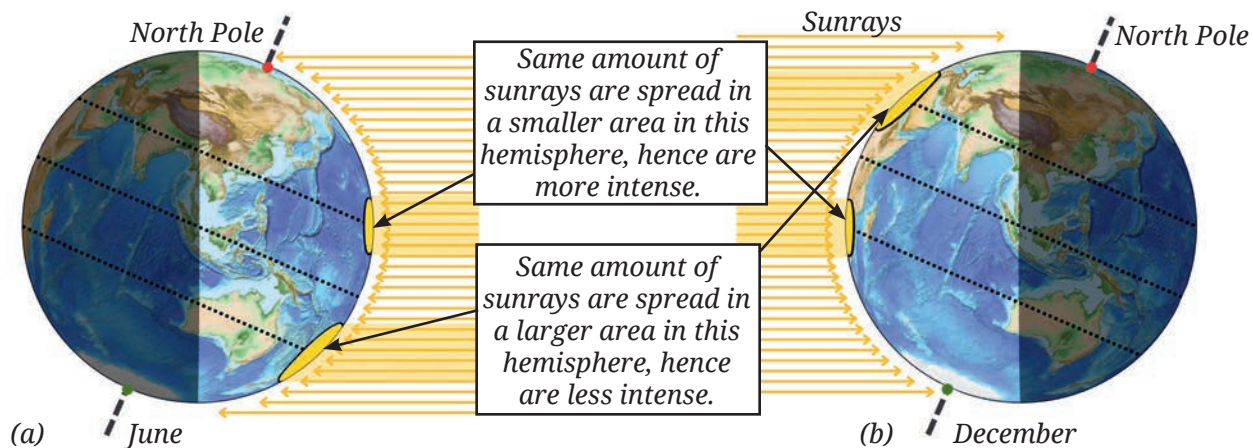
Fig. 12.10: (a) More intense sunlight in the Northern Hemisphere and less intense sunlight in the Southern Hemisphere in June (b) The opposite situation happens in December.
