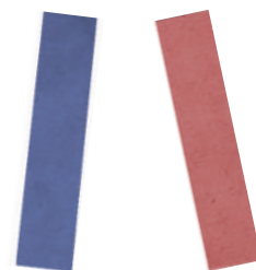
Fig. 2.3: Blue and red litmus paper strips
