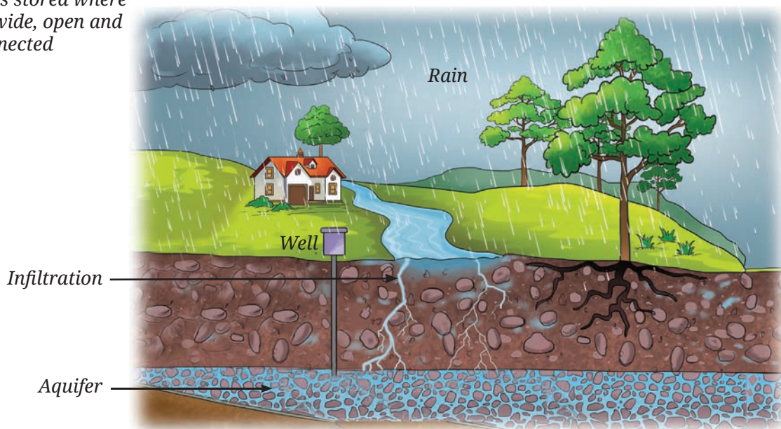
Fig. 7.12: Aquifer
