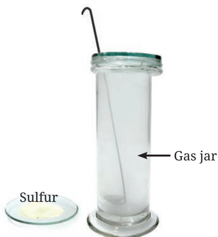
Fig. 4.7(c): Burning of sulfur
