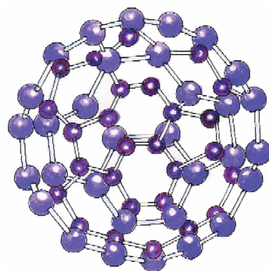
Fig 6.3 Fullerene
