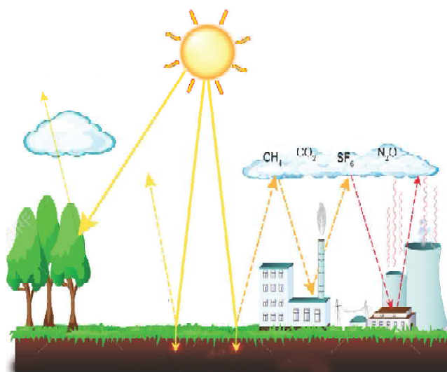
Fig.3.4 Greenhouse effect
