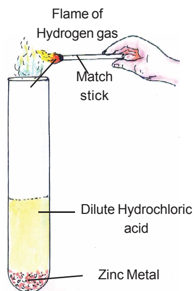
Fig 4.2 Displacement
