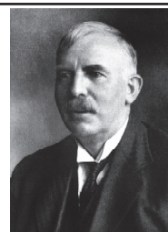
Rutherford
