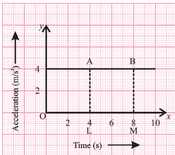
Fig. 8 : Acceleration - Time graph of uniform accelerated motion
