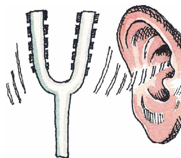
Fig. 3 : Vibrations in a tuning fork
