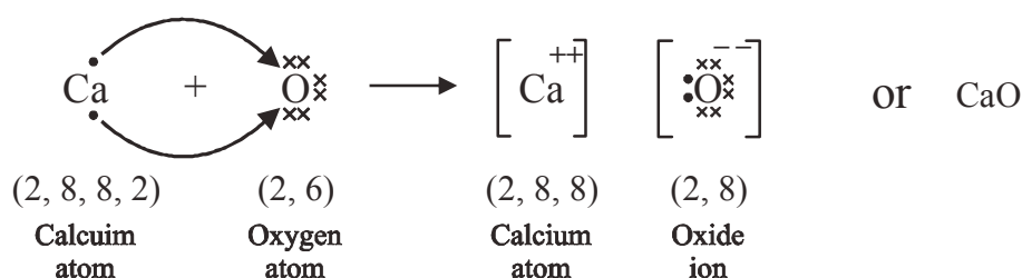
Fig. 3 : Formation of Calcium oxide
