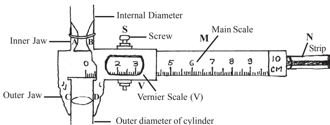
Fig. : Measuring diameter of a glass marble by using a pair of Vernier Callipers
